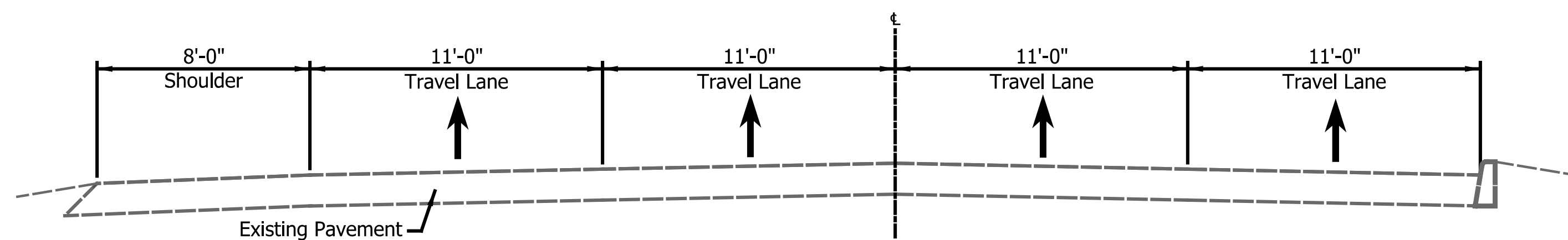
W Kilgore Ave (SR 32) Existing Typical Section
