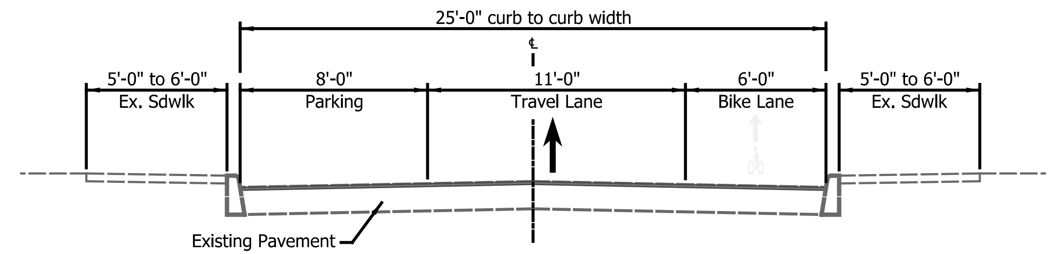
Jackson St. (SR 32) Proposed Typical Section
