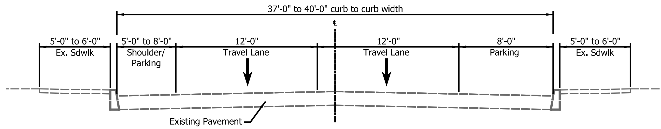
Main St. (SR 32) Existing Typical Section
