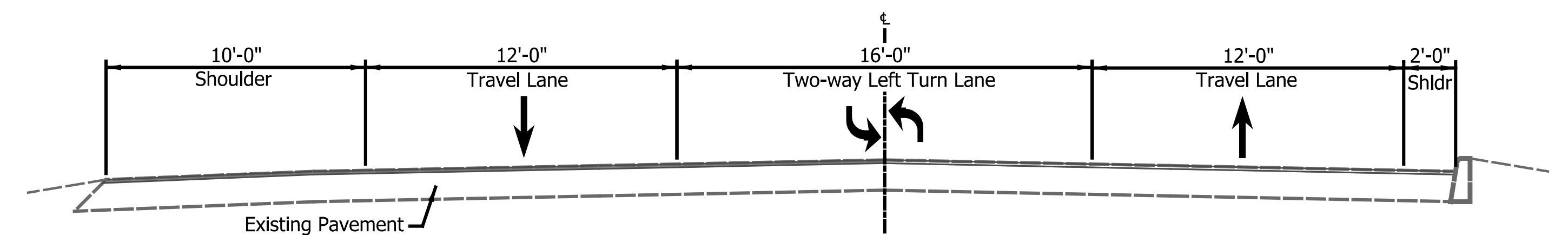
W Kilgore Ave (SR 32) Proposed Typical Section
