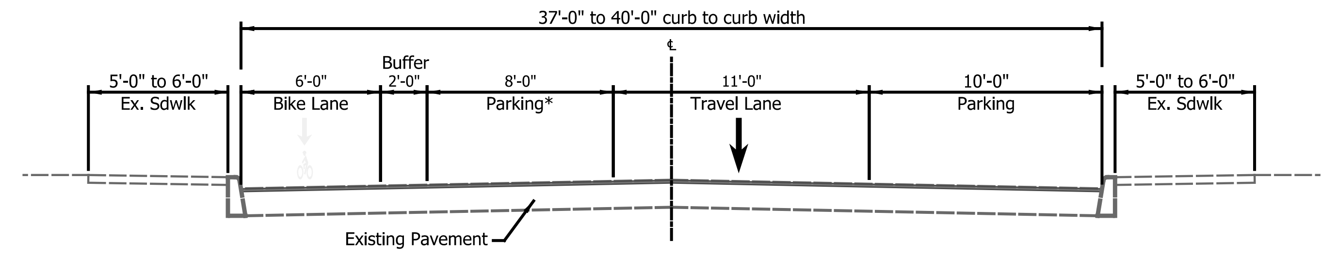
Main St. (SR 32) Proposed Typical Section
