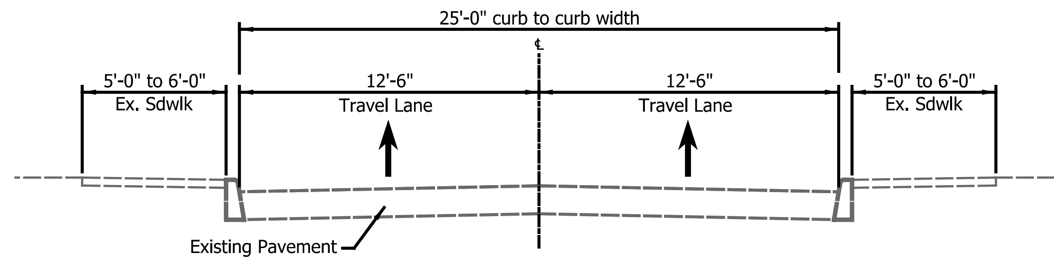
Jackson St. (SR 32) Existing Typical Section
